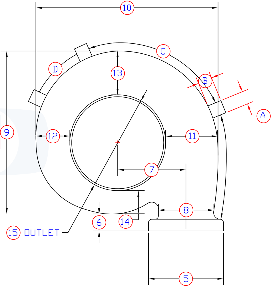
TYPICAL TURBO WITH BOSS DIMENSION SHEET
